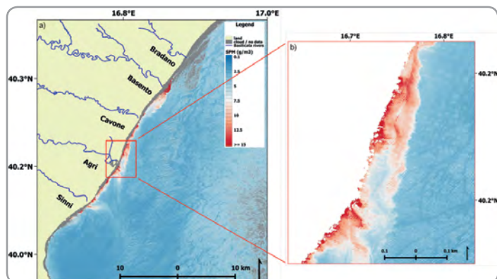
Example of application of MSI-Sentinel-2A data acquired on 30 th April, 2018, for monitoring SPM in the investigated area.
