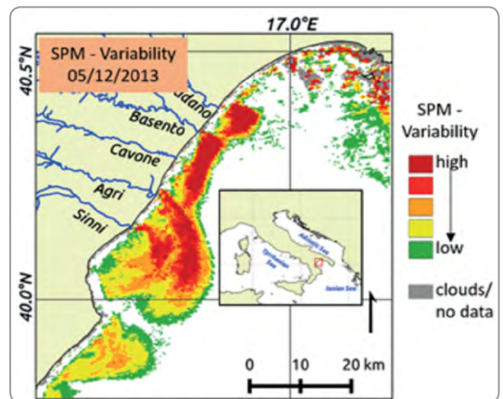
SPM variability for the Basilicata region coastal water area for the MODIS image acquired on 5 December 2013.
